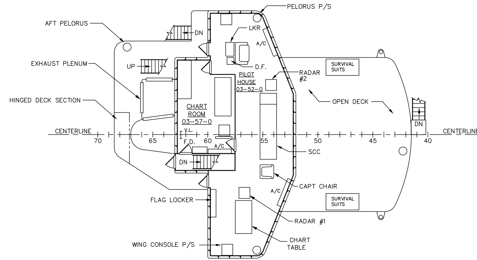
03 LEVEL PLAN
