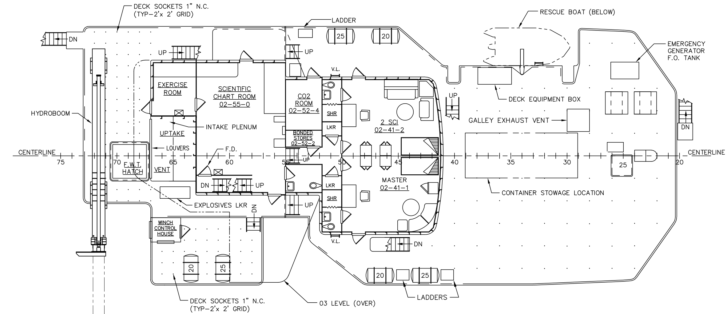
02 LEVEL PLAN
