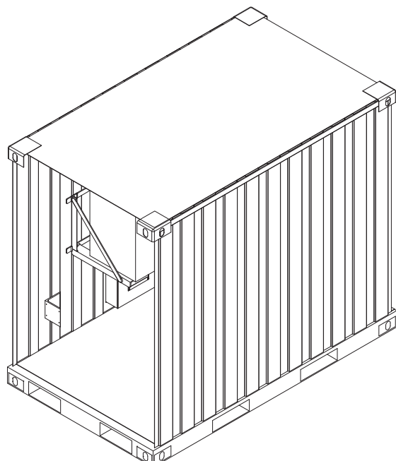
ISO VIEW 5-B DOORS REMOVED FOR CLARITY
